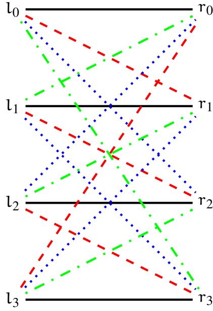
Figure 4.7: The cyclic partition of K_{4,4} is embeddable.
