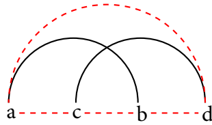
Figure 2.1.: If a < c < b < d occurs for two edges \{a, b\} and \{c, d\} , there is no page embedding with the order < . Especially not a canonical one using semi-circles. The red (dashed) edges result from adding the spine to the page embedding.
