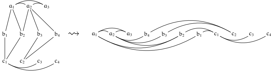
Figure 4.18.: A MULTIPLE-SPINE-EMBEDDING instance can be transformed into a 2-page book embedding instance with separated sets of vertices.
