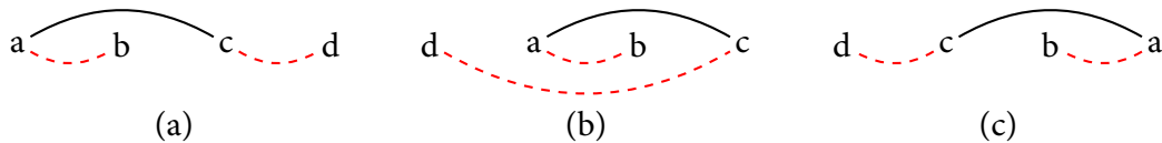
Figure 2.2.: A valid book embedding (a) with cyclic shift to the right by one element (b) and mirror image (c).
