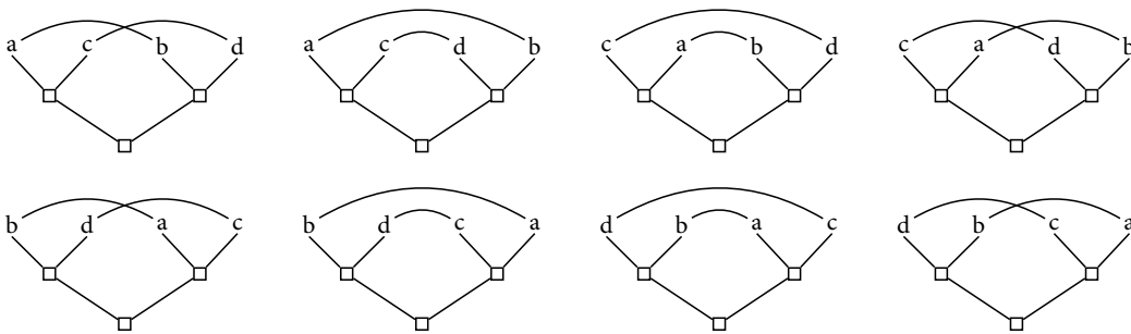
Figure 4.14.: The tree orders for the case outside 1.
