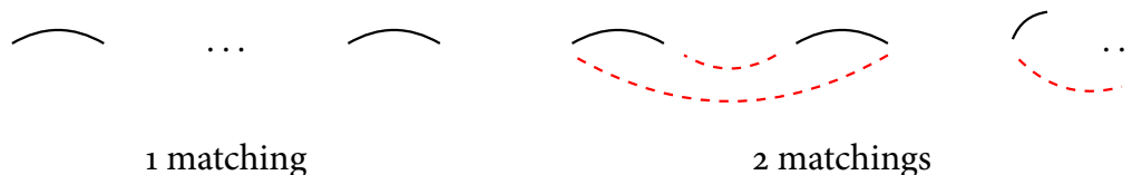
Figure 4.4.: One matching just consists of independent edges, while two matchings form disjoint cycles.
