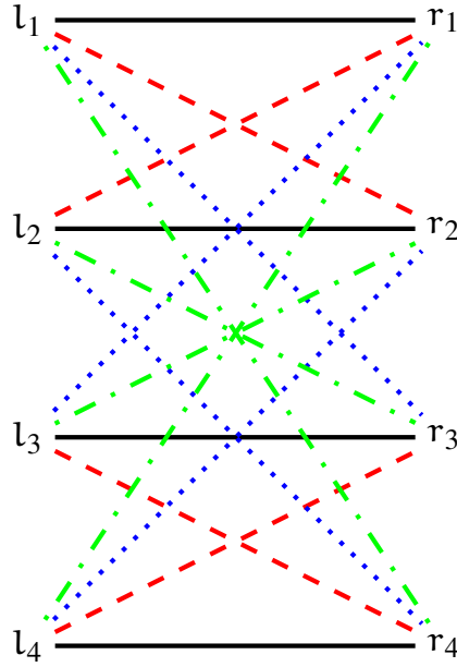
Figure 4.5.: A non-embeddable partition of K_{4,4} .
