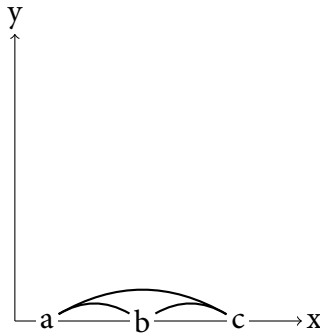
Figure 1.1.: A page embedding of C_3
