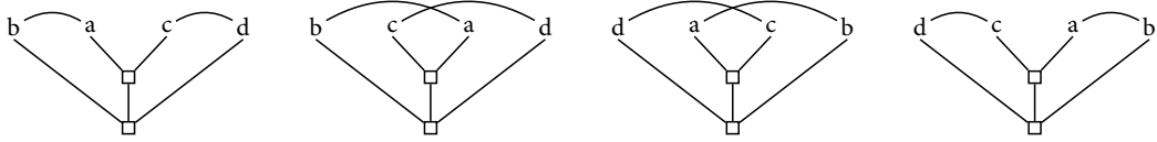
Figure 4.15.: The tree orders for the case inside 1.
