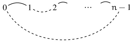
Figure 4.8.: Two matchings form a cycle.
