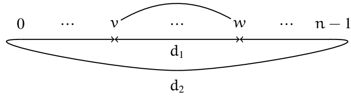
Figure 4.9.: The value \mu(v) = \min\{d_1, d_2\} is the length of the edge \{v, w\} in the symmetric order.
