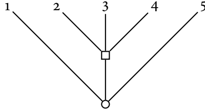
Figure 1.2.: A simple PQ-tree. P-nodes are drawn as a circle \circ , Q-nodes as a box \square .
