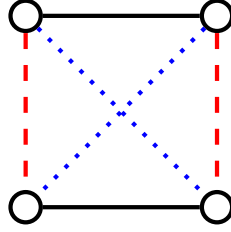
Figure 4.2.: A non-embeddable partition of K_4 .
