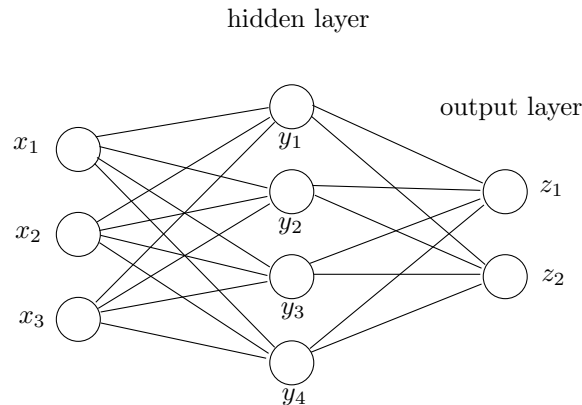
Figure 2.5: multilayer perceptron
