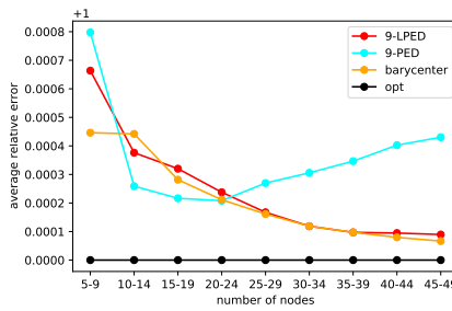
Figure 5.32: performance on the distribution from G(n, n, 0.75) with n \sim U(5, 49)
