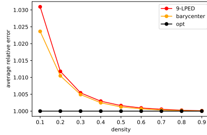
Figure 5.20: performance on the distribution from G(20, 20, p) with p \sim U(5, 95)
