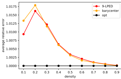
Figure 5.11: performance on the distribution from G(10, 10, p) with p \sim U(5, 95)
