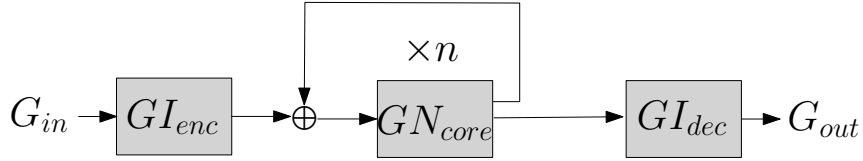
Figure 3.9: Encode-process-decode
